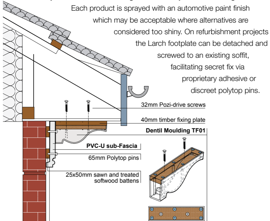
Typical Dentil Installation
